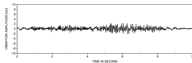
[Gitzo 1227 1.56kg (3.03 lbs) tripod]
