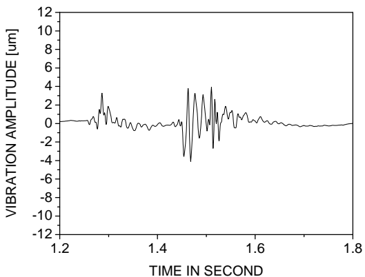
[Hasselblad 205FCC with standard lens]
